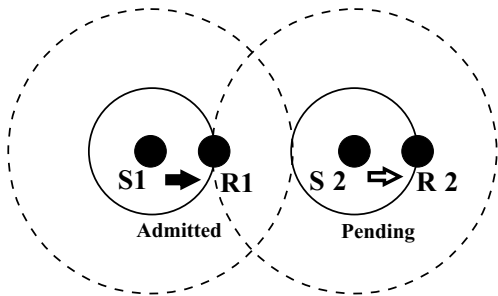
Fig. 14. Scenario likely to cause an erroneous admission control decision using CACP.
