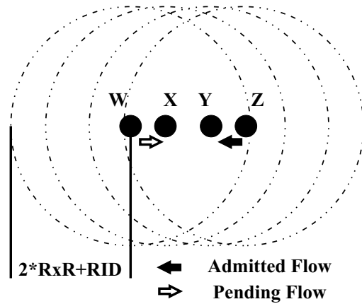
Fig. 9. PAC single-hop admission control decision example.
