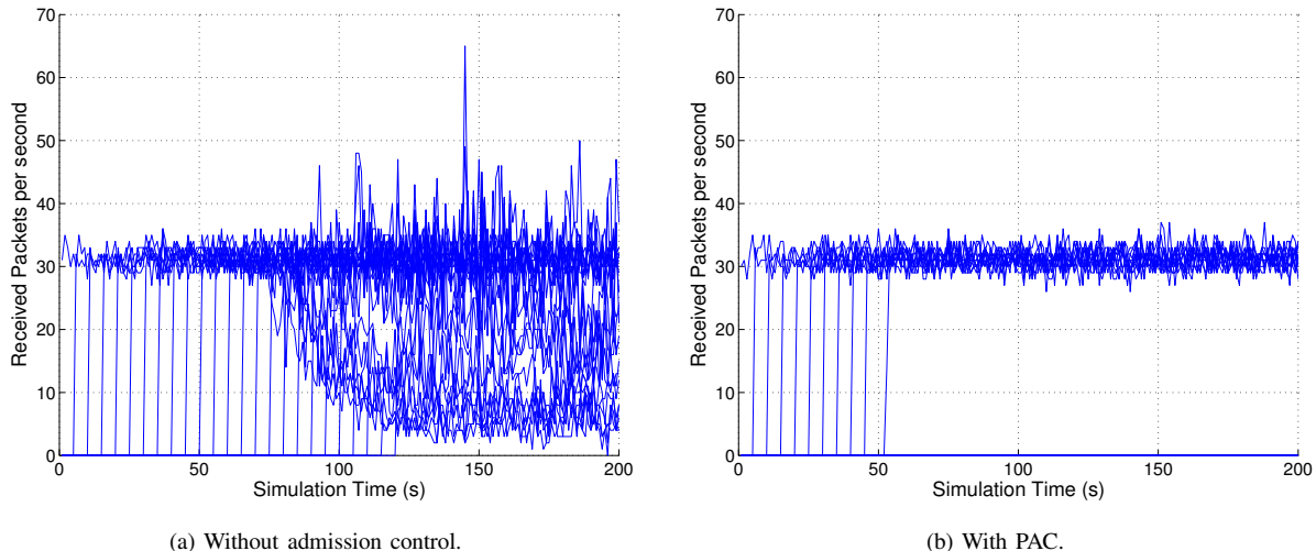
Fig. 13. Throughput for all flows.
