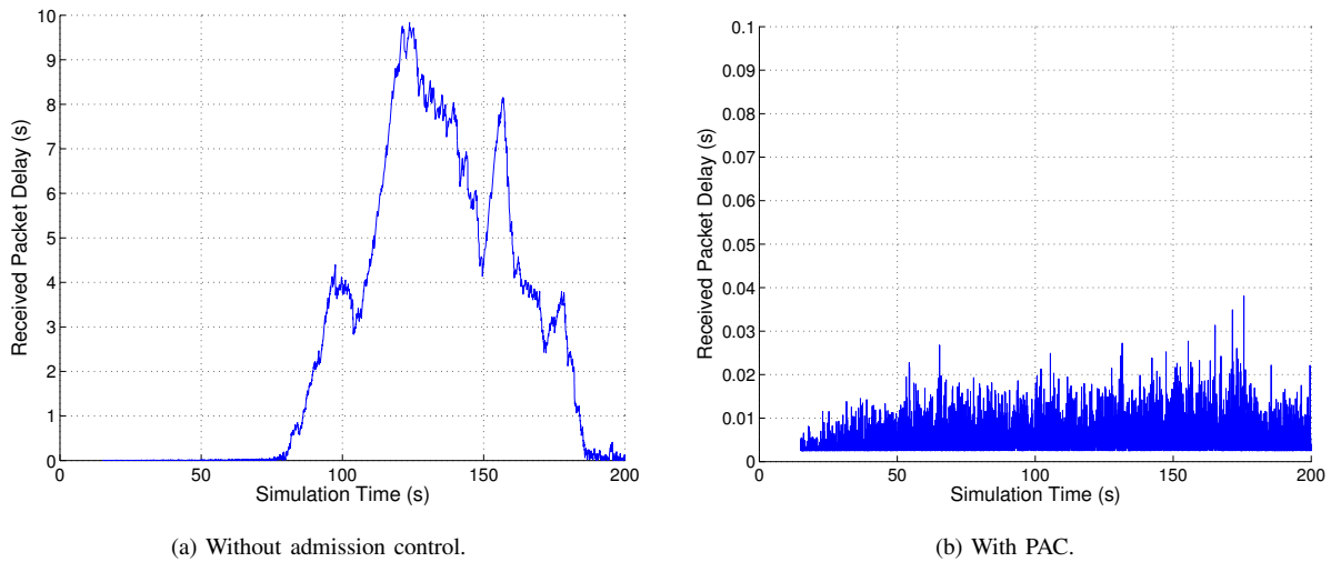
Fig. 12. Delay of a single representative receiver in one simulation.
