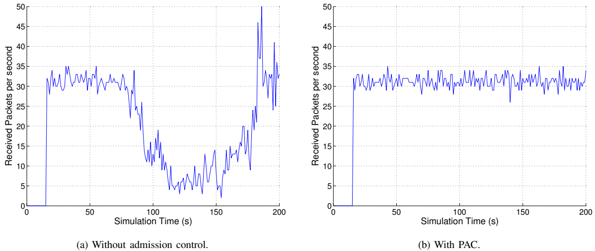
Fig. 11. Throughput of a single representative receiver in one simulation.
