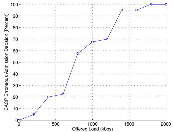
Fig. 15. CACP erroneous admission control decision.
