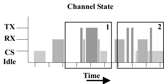
Fig. 4. An example of channel state. At different times a node may be either idle, sensing a packet transmission (CS), receiving a packet (RX) or sending a packet (TX). In window 1 the channel is busy half the time. In window 2 the channel is busy nearly 100%.
