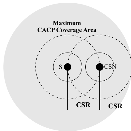
Fig. 16. Maximum CACP coverage area. CACP queries all CSN to check whether there is enough available bandwidth to support a new flow.
