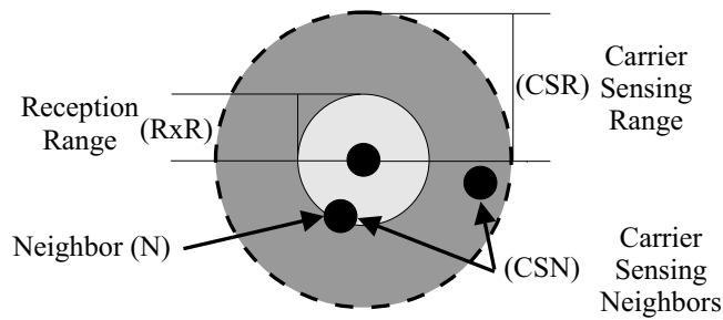
Fig. 1. Approximation of reception range (RxR) and carrier sensing range (CSR). Nodes within reception range are called neighbors (N), while carrier sensing neighbors (CSN) are all nodes within carrier sensing range.
