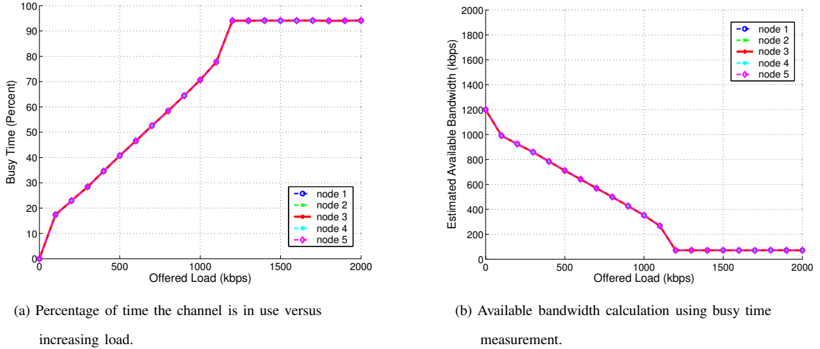
Fig. 6. Simulation results of busy time measurement technique.
