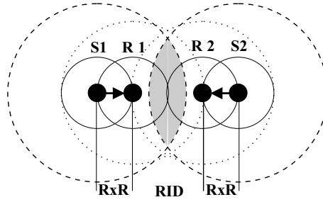
Fig. 3. Spacing requirement for simultaneous transmissions in wireless networks that utilize acknowledgments. Since the sender's RID and receiver's CSR are not important to the interference calculation, they are not shown.
