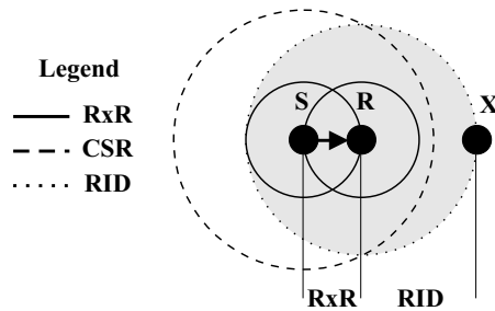
Fig. 2. The receiver interference distance (RID) is the distance between a receiver (R) and another sender (X), such that the receiver can successfully receive S's packets and X can simultaneously send a packet to another receiver.
